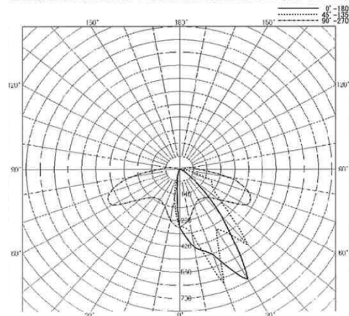
LUMINOUS INTENSITY DISTRIBUTION CURVE (cd/1000lm)
